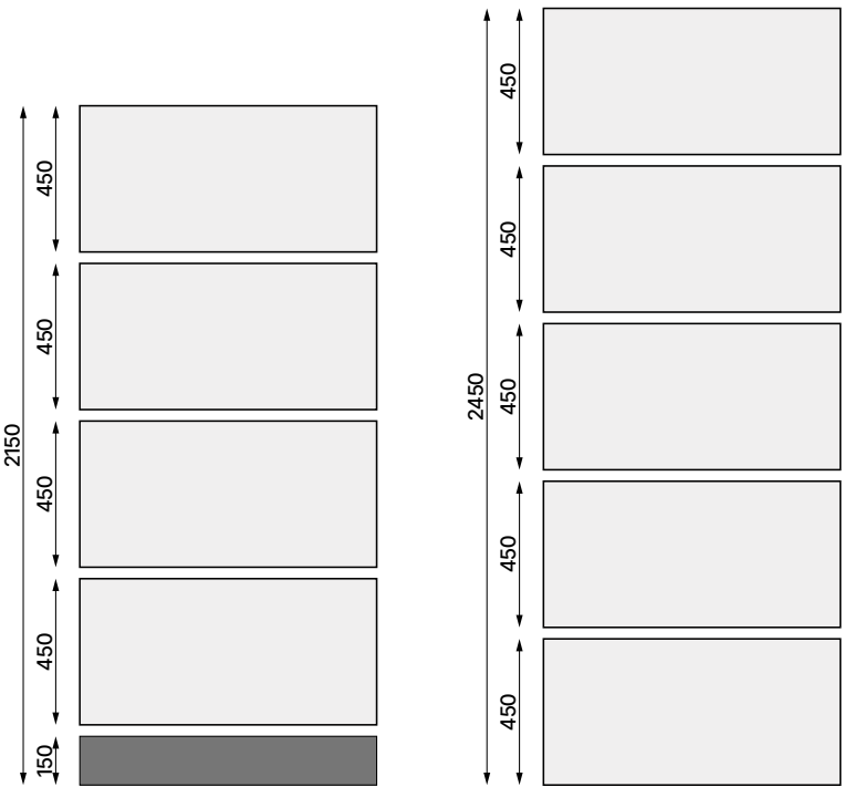
Punch Panel Sizing Diagram
