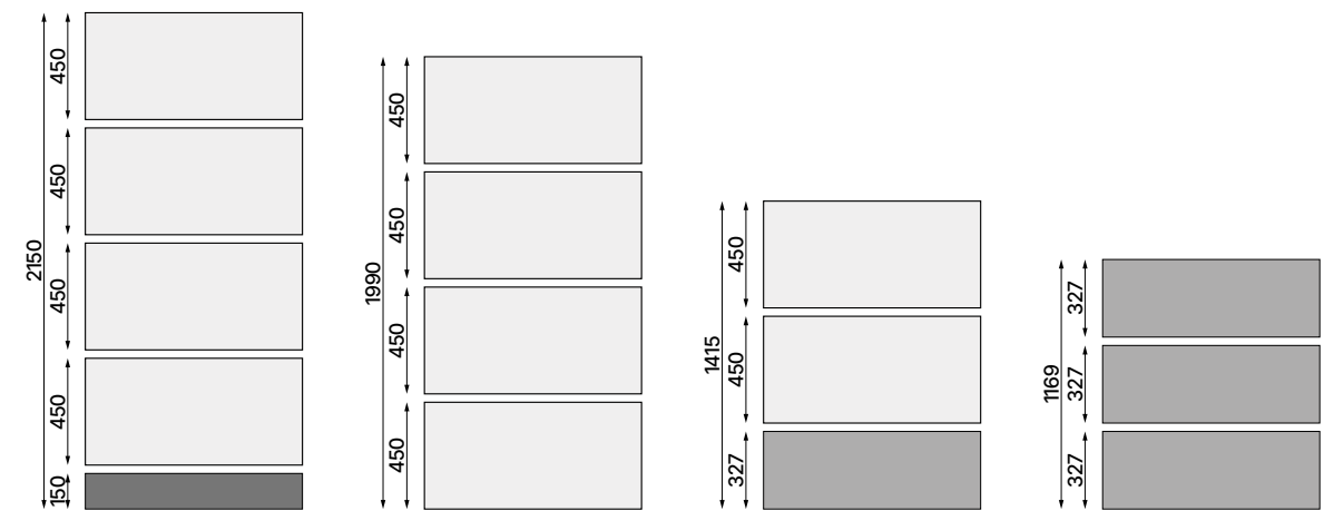
Punch Panel Sizing Diagram
